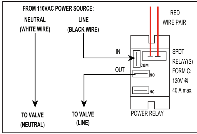
EXAMPLE OF CONNECTING A 110VAC SOLENOID VALVE
